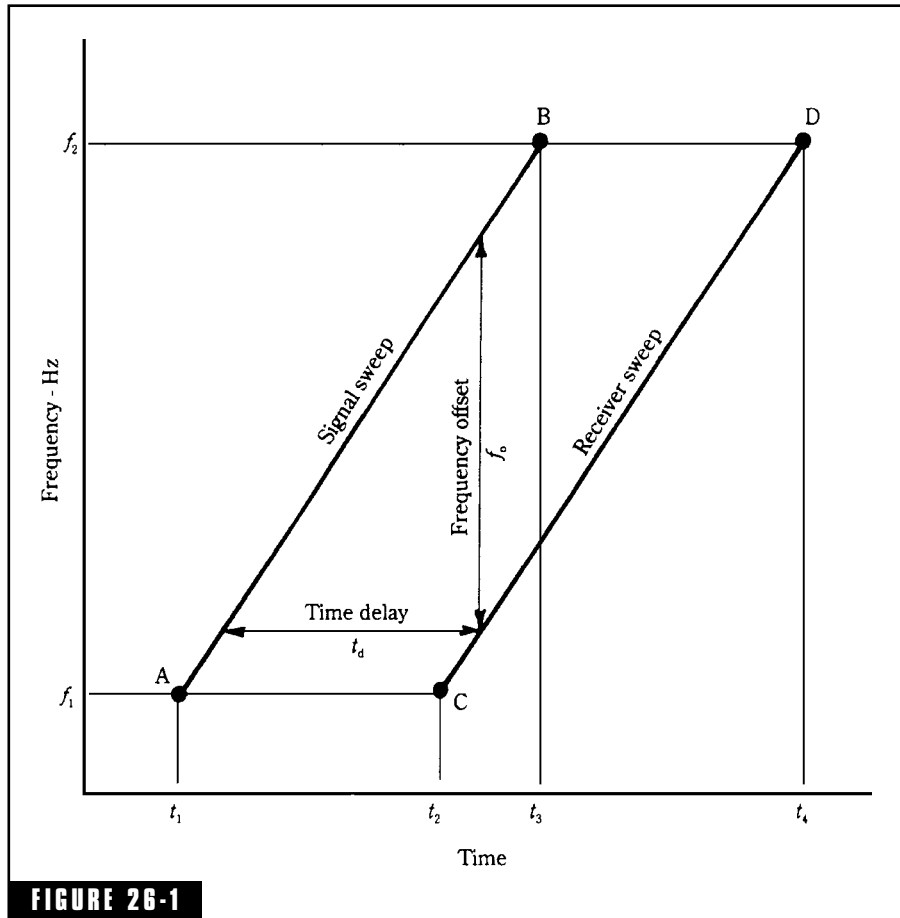
FIGURE 26-1 The basic principles of Heyser's time-delay spectrometry measurements. The outgoing signal is swept linearly from A to B. After a delay appropriate to select out the reflection desired, the receiver is swept from C to D. Only energy from the desired reflection is accepted; the receiver is detuned to all others.
