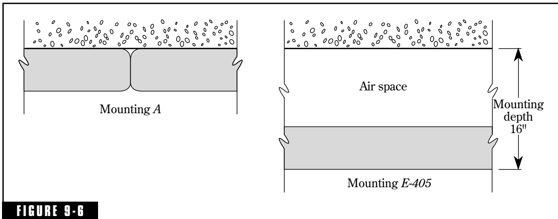
FIGURE 9-6 Commonly used standard mountings associated with listings of absorption coefficients. With Mounting A the material is flat against the backing. Mounting B (not shown) is similar to Mounting A but with a \frac{1}{16} " air-space resulting when acoustical materials are cemented to a surface. Mountings B and A are essentially the same. Mounting E-405 applies to suspended ceilings with lay-in panels. (See Table 9-1.)
