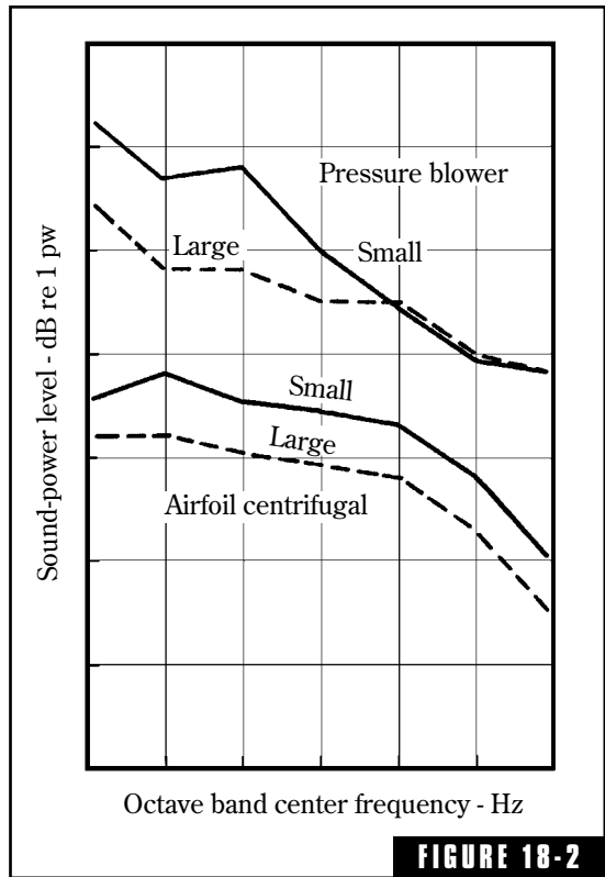
FIGURE 18-2 Noise sound-power output of different types of fans commonly used for air-conditioning. (Data are from Table 22-2. 2 )
