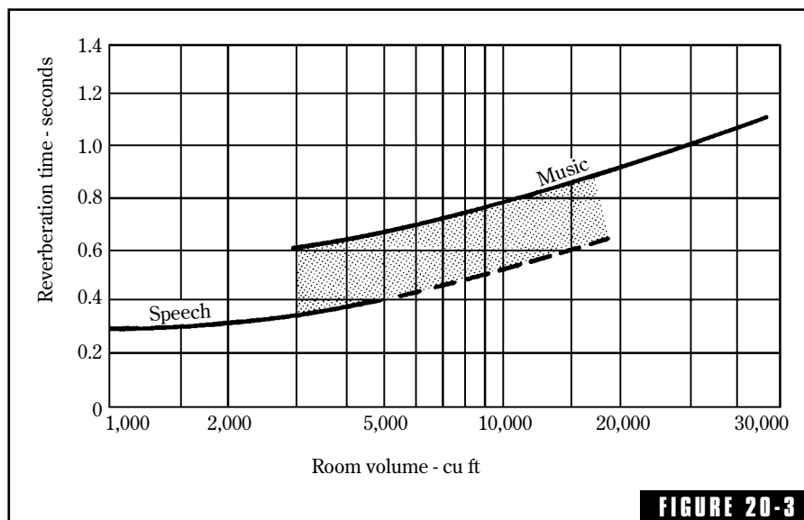
FIGURE 20-3 Suggested reverberation times for recording studios. The shaded area is a compromise region for studios in which both music and speech are recorded.
