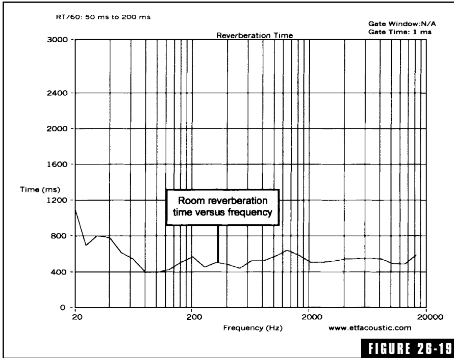
Room reverberation chart showing measured RT/60 values at various frequencies. (Courtesy of Doug Plumb, AcustiSoft.)
