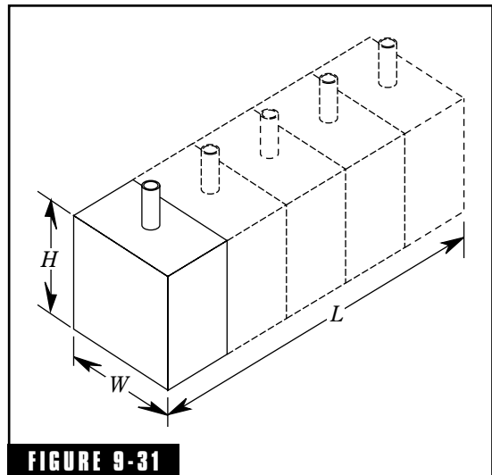
FIGURE 9-31 Development of perforated-face Helmholtz resonator from a single rectangular-bottle resonator.
