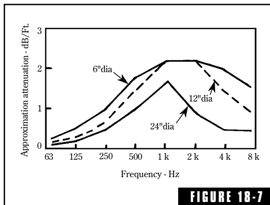
Attenuation offered by spiral wound round ducts with perforated spiral wound steel liner. Dimensions shown are the free area inside the duct, with no air flow. This is a plot of the data from Ref.2.
