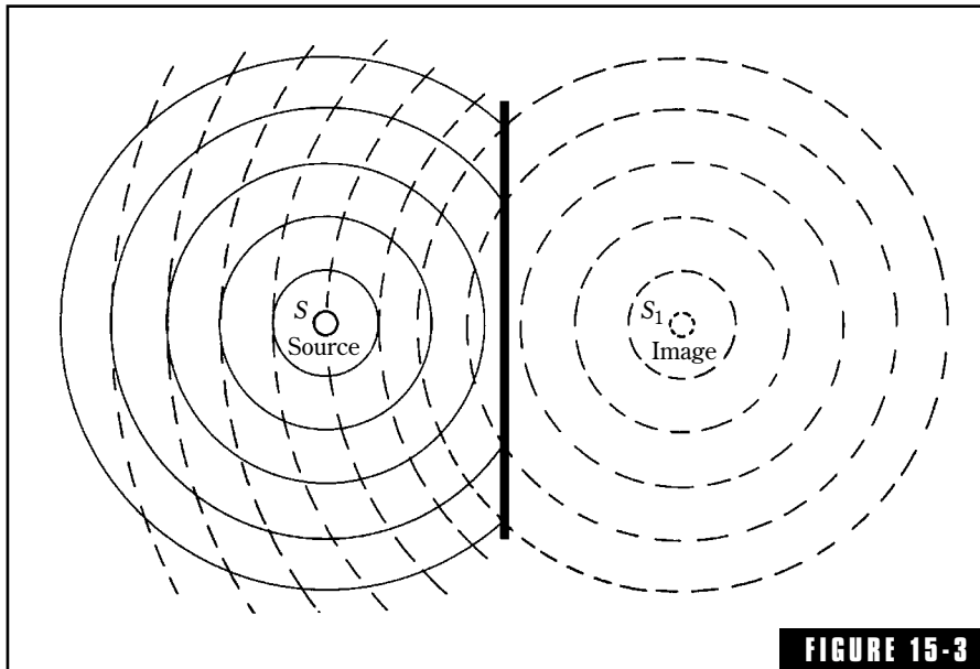
FIGURE 15-3 Sound radiated by a point S is reflected by the rigid wall. The reflected wave can be considered as coming from S_1 , an image of S .
