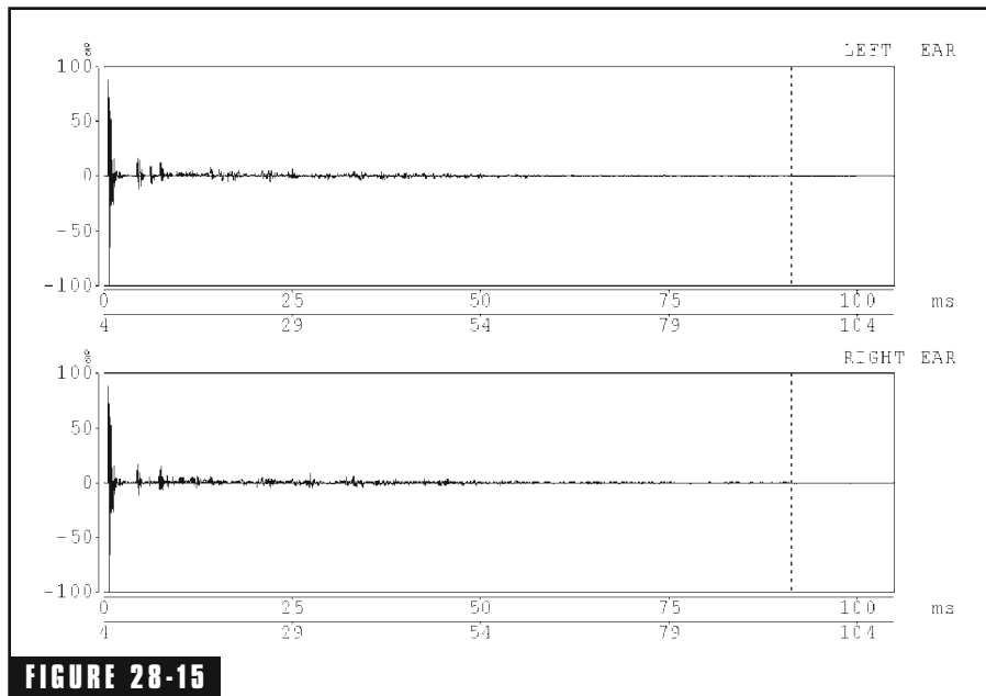
Convolution of the echogram reflections with the HRTFs results in a binaural room impulse response shown for the left ear (top) and right ear (bottom).
