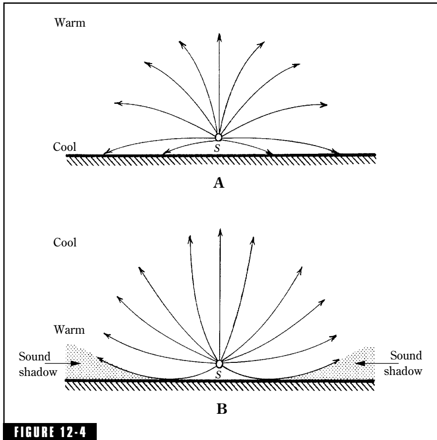
FIGURE 12-4 Comprehensive illustration of refraction of sound from source S ; (A) cool air near the ground and warmer air above, (B) warm air near the ground and cooler air above. In (B) note that sound shadow areas result from the upward refraction.
