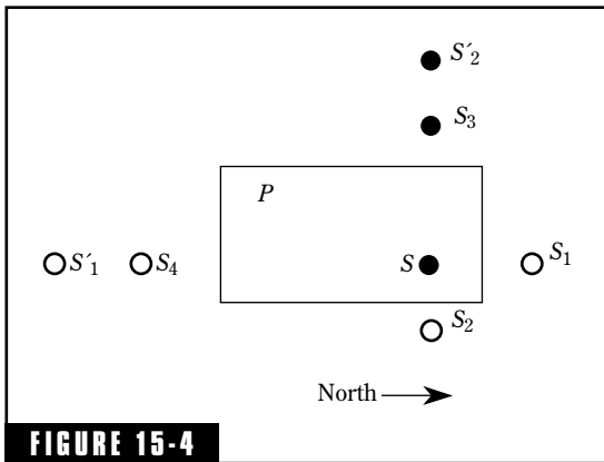
FIGURE 15-4 The surface of Fig. 15-3 is now made into the north wall of an enclosure. The source S now has six primary images, one in each of the six surfaces of the enclosure. Images of the images result in a theoretically infinite number of images of S . Sound intensity at point P is made up of the direct sound from S plus the contributions from all images.
