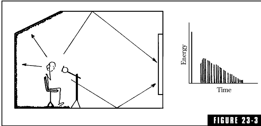
FIGURE 23-3 Voice booth for high-quality sound. Early reflections are eliminated by the absorbent rear end and the diffusor assures a dense ambient decay.
