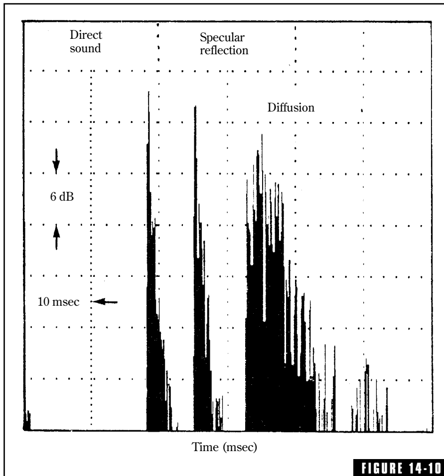
FIGURE 14-10 An energy-time contrast of a specular reflection from a flat panel and the energy diffused from a quadratic residue diffusor. The peak energy from a diffusing surface is somewhat lower than that of the flat panel but it is spread out in time. Peter D'Antonio, RPG Diffusor Systems, Inc. and the Audio Engineering Society.
