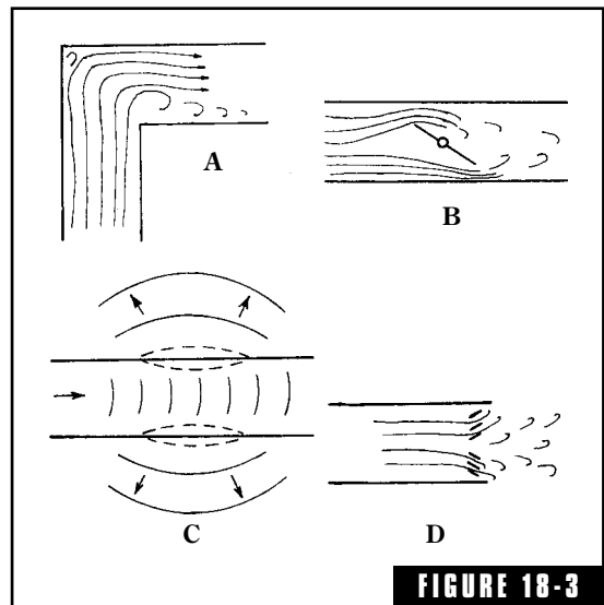
FIGURE 18-3 Air turbulence caused by discontinuities in the flow path can be a serious producer of noise. (A) 90-degree miter bend. (B) Damper used to control quantity of air. (C) Sound radiated from duct walls set into vibration by turbulence or noise inside the duct. (D) Grilles and diffusers.
