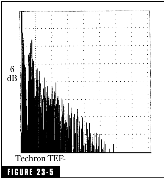
FIGURE 23-5 Energy-time-curve (ETC) of the Quick Sound Field™ studio. About 1,000 reflections per second are produced in such a space resulting in a dense, but rapidly decaying ambient field. The horizontal time base goes to 80 ms. Acoustic Sciences Corporation.
