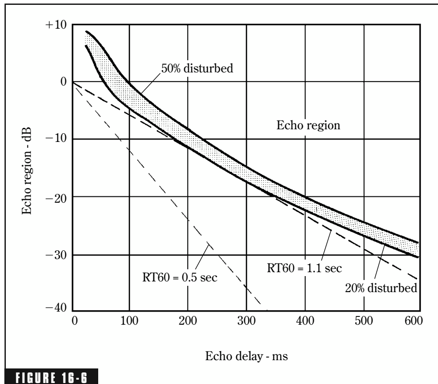
FIGURE 16-6 Acceptable echo levels for speech under reverberant conditions (Reverberation Time 1.1 seconds). After Nickson, Muncey, and Dubout. 4
