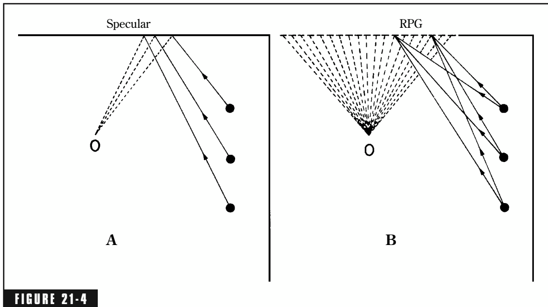
FIGURE 21-4 The three black spots represent side-wall reflection in a control room returning energy to the operator, O . If the rear wall is specular, only a single point on the rear wall returns energy to the operator. Each element of a reflection-phase-grating diffusor returns energy to the operator. Peter D'Antonio, RPG Diffusor Systems, Inc., and Audio Engineering Society, Inc.
