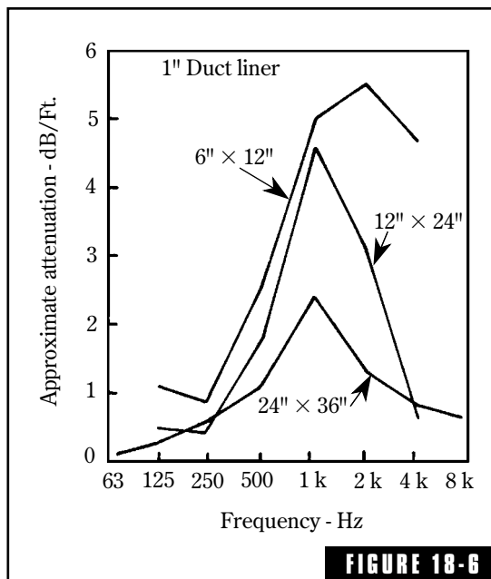
Attenuation offered by 1" duct lining on all four sides of rectangular duct. Dimensions shown are the free area inside the duct with no air flows. This is a plot of the data from Ref.2.
