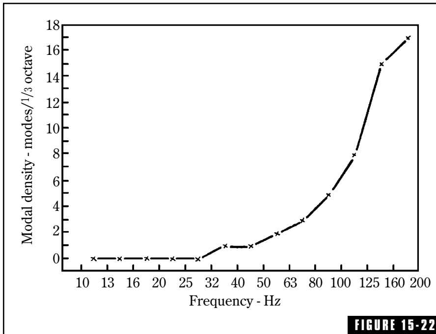
FIGURE 15-22 A plot showing the number of modes in 1/3 octave bands for the 15.4 X 12.8 X 10 ft room. The graph climbs steadily upward with no downward anomalies; hence the room meets the Bonello criterion.
