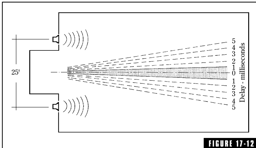
FIGURE 17-12 In the common split system in which two loudspeakers radiate identical signals, zones of constructive and destructive interference result which degrade sound quality in the audience area.
