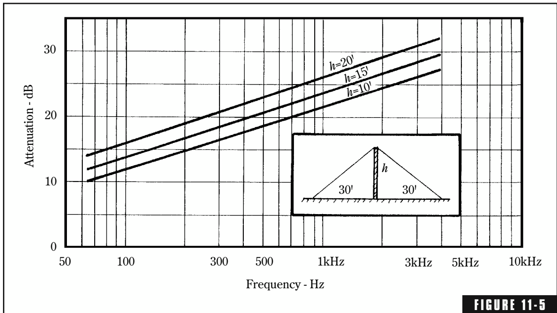
FIGURE 11-5 An estimation of the effectiveness of a sound barrier in terms of sound (or noise) attenuation as a function of frequency and barrier height. (After Rettinger. 4 )
