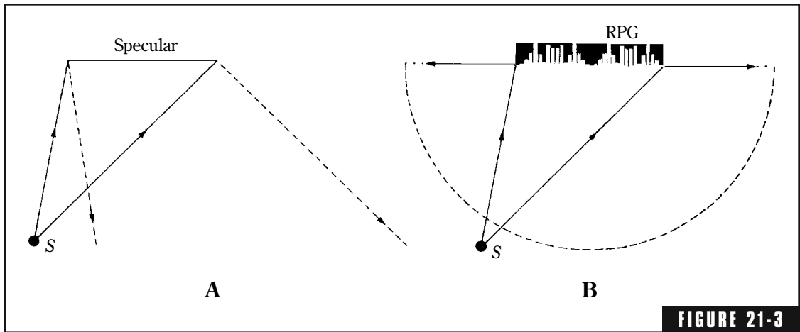
FIGURE 21-3 A comparison of reflection of sound energy from (A) a flat surface, which yields specular reflection, and (B) a reflection-phase grating, which yields energy dispersed in a hemidisc. Peter D'Antonio, RPG Diffusor Systems, Inc., and Audio Engineering Society, Inc.
