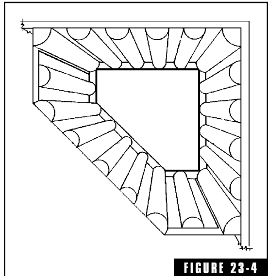
FIGURE 23-4 View of small voice-over studio based on the Quick Sound Field™ idea. The ceiling, walls, door, and the observation window are all covered with spaced half-round Tube Traps™. Acoustic Corporation.
