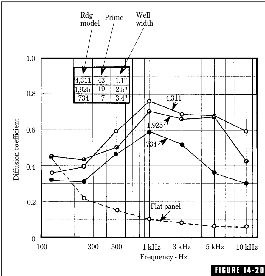
FIGURE 14-20 Comparison of the variation of diffusion coefficient with frequency of three RPG™ dif- fusers and a flat panel. Peter D'Antonio, RPG Diffusor Systems, Inc.
