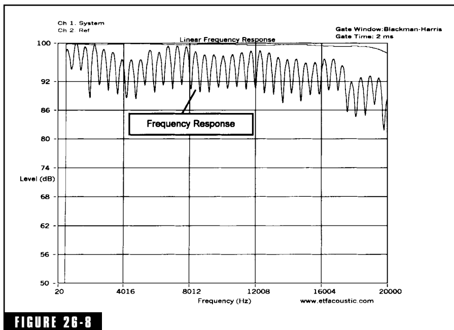
Frequency response of a loudspeaker measured at a distance of 1 m, with a single reflecting surface nearby. (Courtesy of Doug Plumb, AcustiSoft.)
