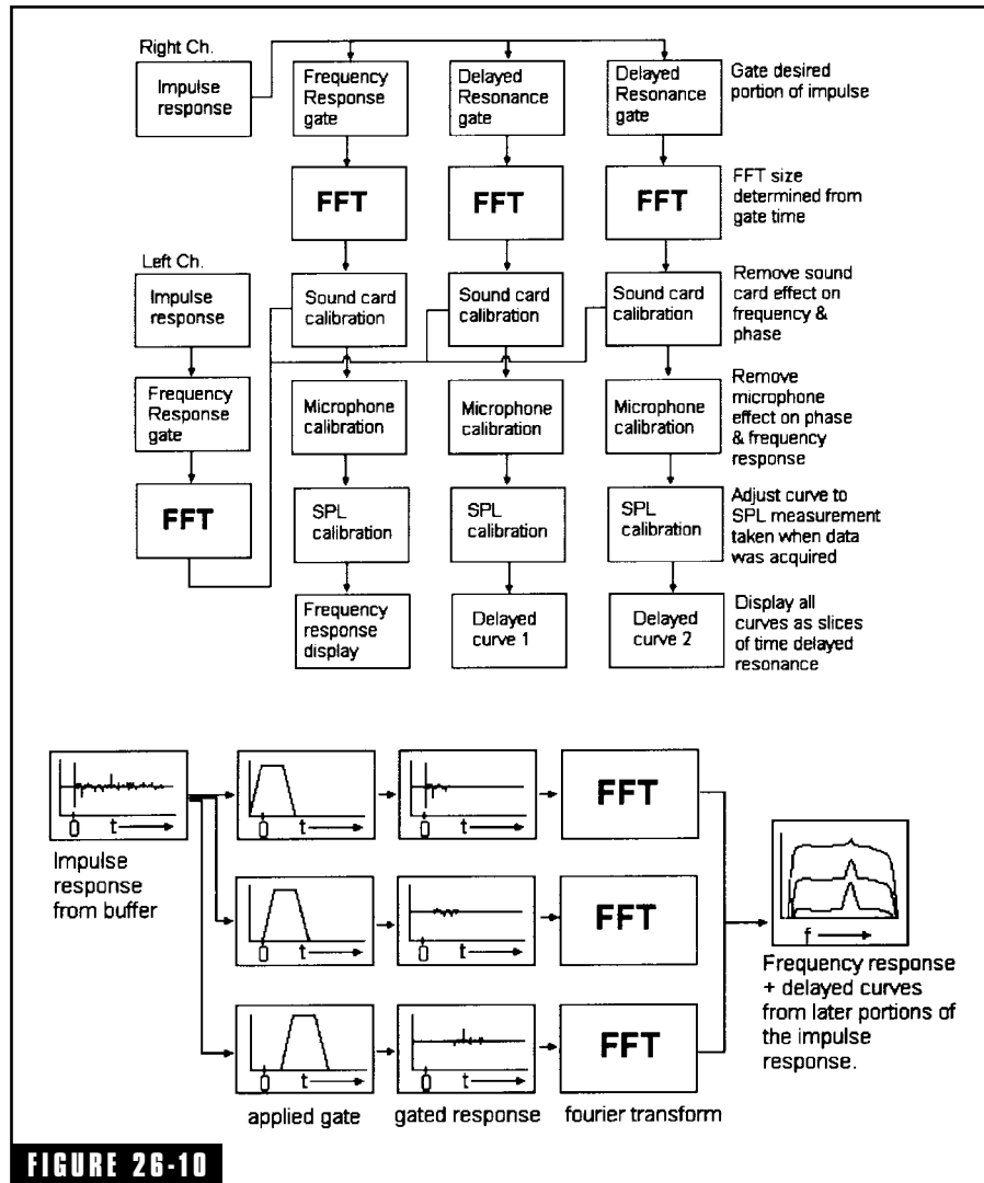
Block diagram of ETF 5's time slice frequency response computation methodology. (Courtesy of Doug Plumb, AcustiSoft.)
