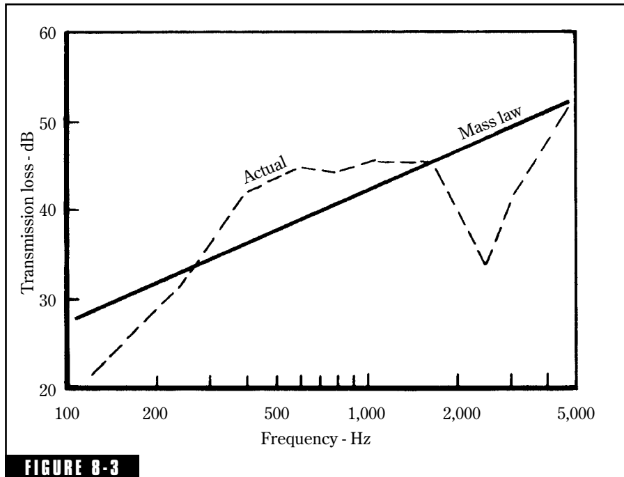
FIGURE 8-3 Actual measurements of transmission loss in walls often deviate considerably from the mass law (Fig. 8-2) because of resonances and other effects.
