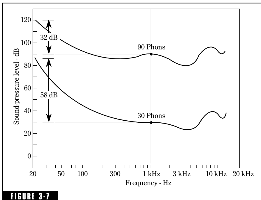
A comparison of the ear's response at 20 Hz compared to that at 1,000 Hz. At a loudness level of 30 phons, the sound-pressure level of a 20-Hz tone must be 58 dB higher than that at 1,000 Hz to have the same loudness. At 90 phons loudness level, an increase of only 32 dB is required. The ear's response is somewhat flatter at high loudness levels. Loudness level is only an intermediate step to true subjective loudness as explained in the text.
