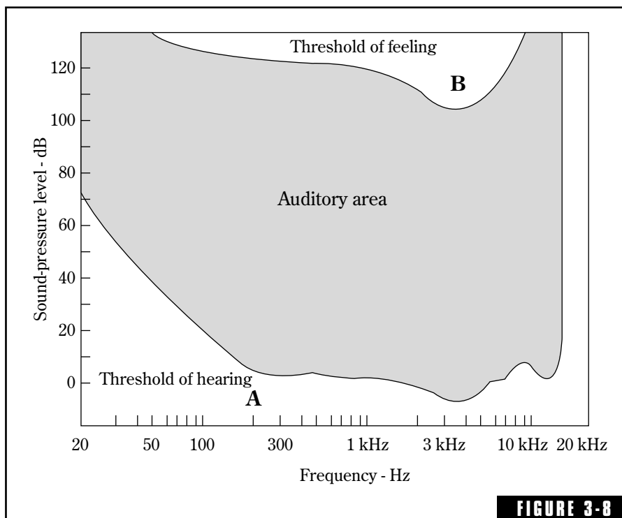
FIGURE 3-8 The auditory area of the human ear is bounded by two threshold curves, (A) the threshold of hearing delineating the lowest level sounds the ear can detect, and (B) the threshold of feeling at the upper extreme. All of our auditory experiences occur within this area.
