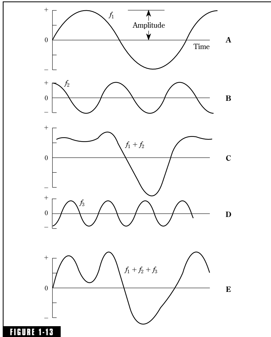
A study of the combination of sine waves that are not in phase. (A) The fundamental of frequency f_1 . (B) The second harmonic f_2 with twice the frequency and half the amplitude of f_1 advanced 90 degrees with respect to f_1 . (C) The combination of f_1 and f_2 obtained by adding ordinates point by point. (D) The third harmonic f_3 with phase 90 degrees behind f_1 , and with half the amplitude of f_1 . (E) The sum of f_1 , f_2 , and f_3 . Compare this waveshape with that of Fig. 1-11(E). The difference in waveshapes is due entirely to the shifting of the phase of the harmonics with respect to the fundamental.
