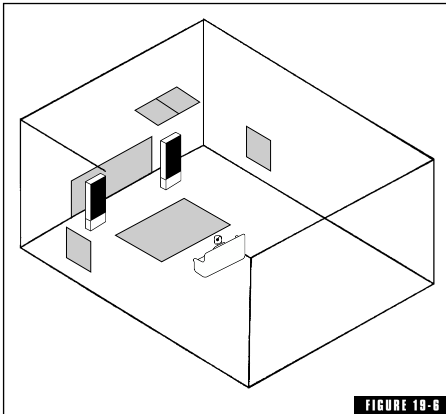
The room of Fig. 19-1 with minimum sound absorbing treatment to reduce the level of the early reflections from room surfaces. The reflectivity of the side-wall absorbers may be adjusted to control spaciousness and image effects in the listening room. Additional absorbing material may be needed to adjust the average reverberant character of the room for best listening.
