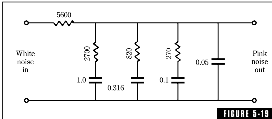
A simple filter for changing white noise to pink noise. It changes random noise of constant energy per Hz to pink noise of constant energy per octave. Pink noise is useful in acoustical measurements utilizing analyzers having passbands with bandwidth of a constant percentage of the center frequency. General Radio Company 1
