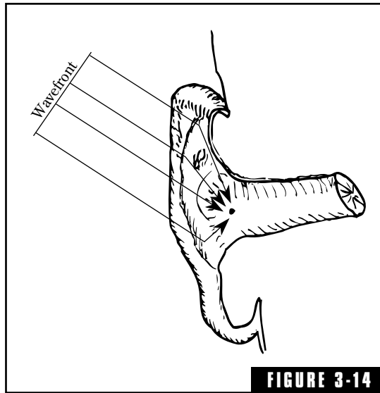
FIGURE 3-14 A wavefront of a sound can be considered as numerous rays perpendicular to that wavefront. Such rays, striking a pinna, are reflected from the various ridges and convolutions. Those reflections directed to the opening of the ear canal combine vectorially (according to relative amplitudes and phases). In this way the pinna encodes all sound falling on the ear with directional information, which the brain decodes as a directional perception.
