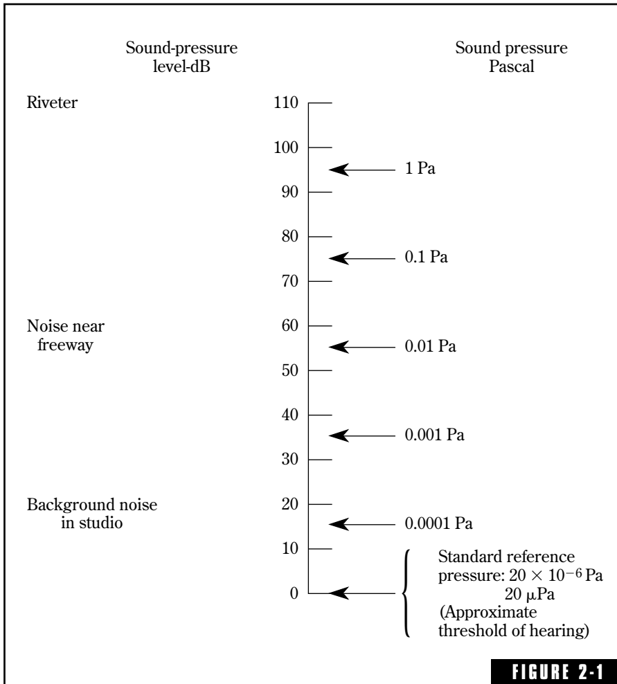
FIGURE 2-1 An appreciation of the relative magnitude of a sound pressure of 1 Pascal can be gained by comparison to known sounds. The standard reference pressure for sound in air is 20\mu\text{Pa} , which corresponds closely to the minimum audible pressure.
