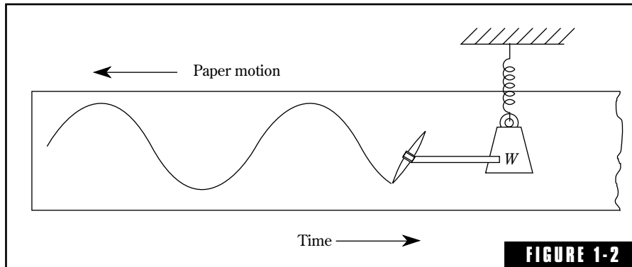
A ballpoint pen fastened to the vibrating weight traces a sine wave on a paper strip moving at uniform speed. This shows the basic relationship between simple harmonic motion and the sine wave.
