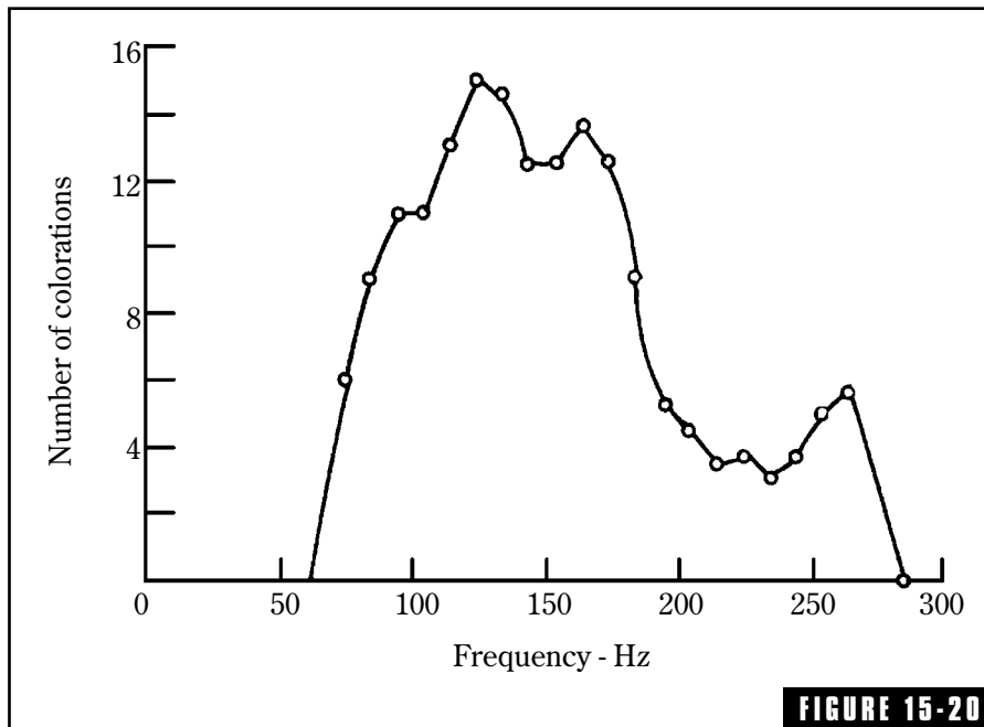
FIGURE 15-20 A plot of 61 male voice colorations observed over a period of 2 years in BBC studios. Most fall in the 100-175 Hz region. Female voice colorations occur between 200 and 300 Hz.
