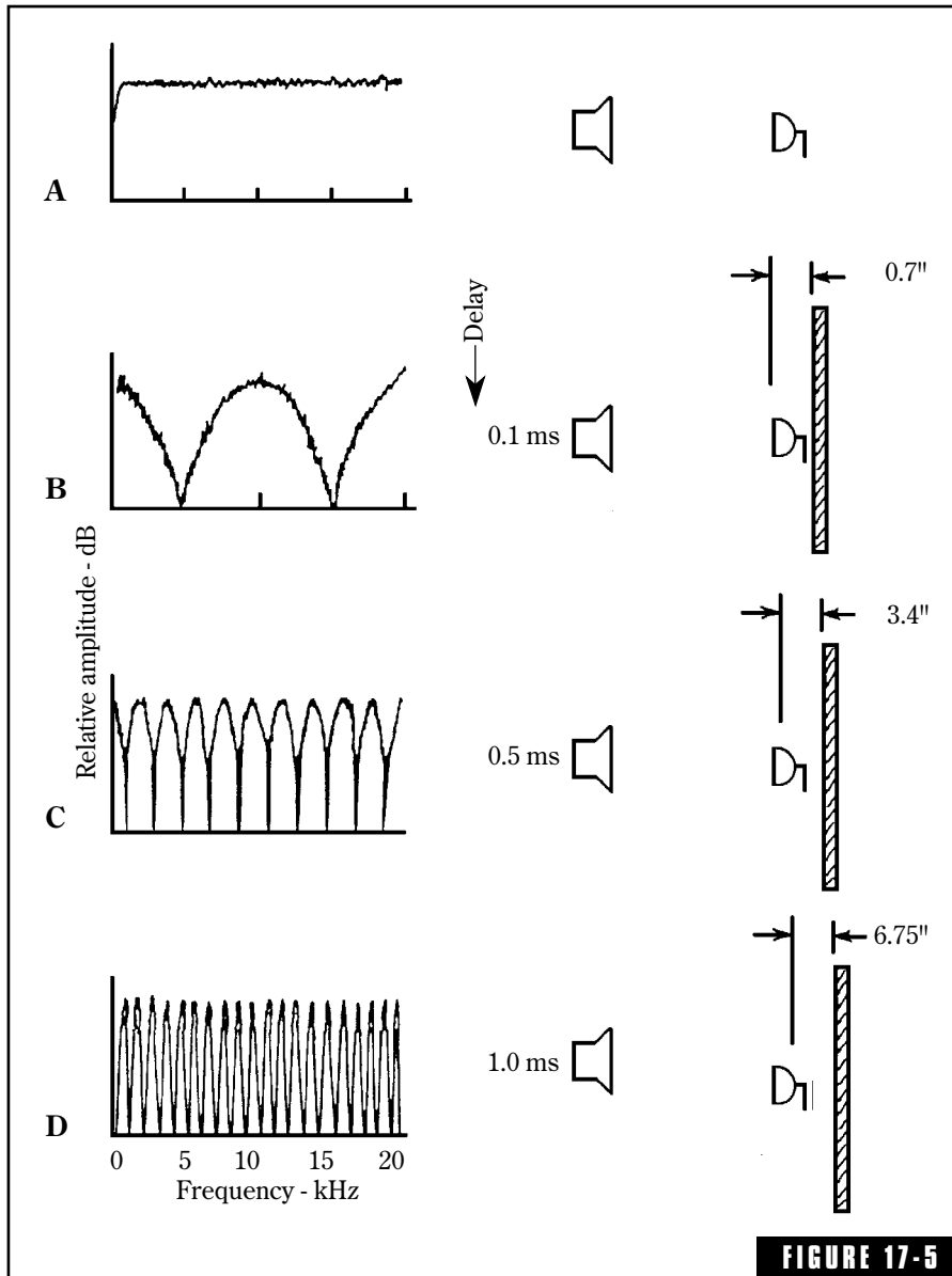
A demonstration of comb filtering in which direct sound from a loudspeaker is acoustically combined with a reflection from a surface at the diaphragm of a microphone. (A) No surface, no reflection. (B) Placing the microphone 0.7 in from the surface creates a delay of 0.1 ms and the combination of the direct and the reflected rays shows cancellations at 5 and 15 kHz and every 10 kHz. (C) A delay of 0.5 ms creates cancellations much closer together. (D) A delay of 1 ms results in cancellations even more closely together. If t is taken as the delay in seconds, the first null is 1/2t and spacing between nulls or between peaks is 1/t .
