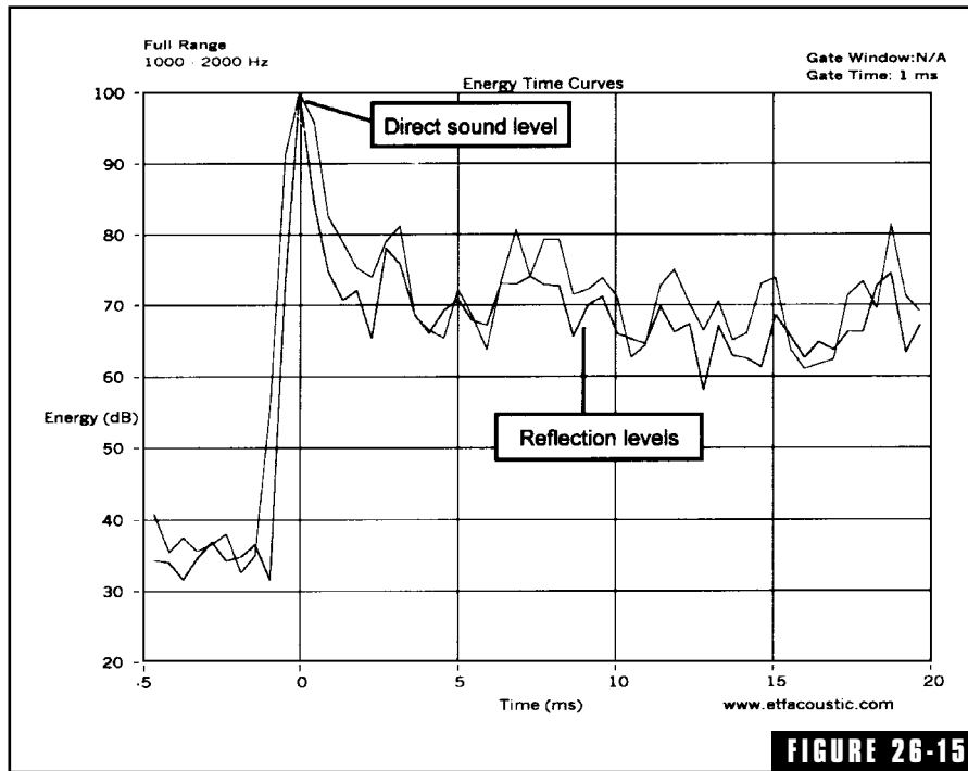
Energy-time curve of a loudspeaker measured at 1 m distance with minimal reflections. (Courtesy of Doug Plumb, AcoustiSoft.)
