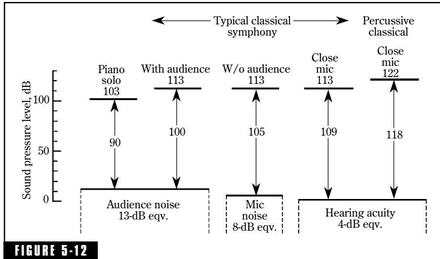
Fiedler's study 6 has shown that a dynamic range of up to 118 dB is necessary for subjectively noise-free reproduction of music.
