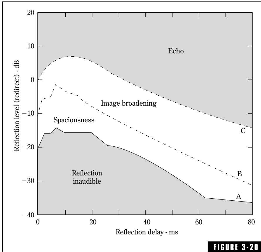
The effects of lateral reflections on the perception of the direct sound in a simulated stereo arrangement. These measurements were made in anechoic conditions, lateral angles 45–90 degrees, with speech as the signal. (A) Absolute threshold of audibility of the reflection. (B) Image shift/broadening threshold (A & B After Olive and Toole, 22 and Toole. 23 ) (C) Lateral reflection perceived as a discrete echo (After Meyer and Schodder, 24 and Lochner and Burger 25 ).
