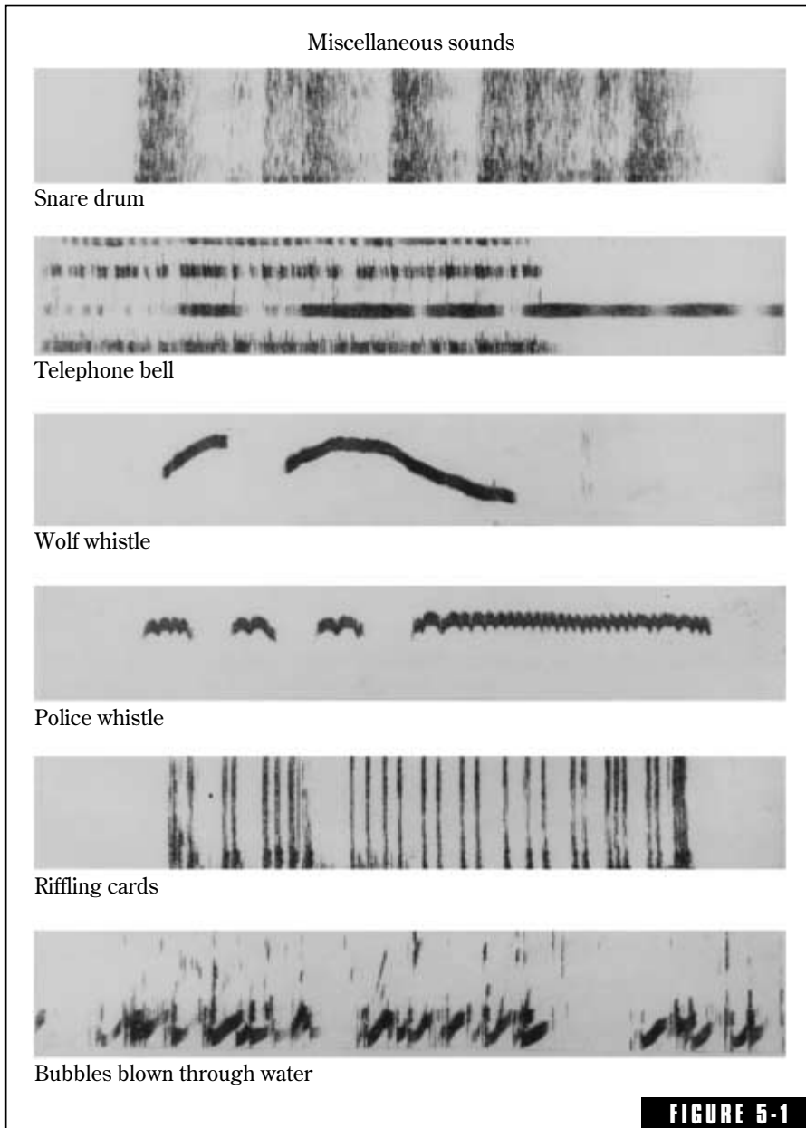
Sound spectrographic recordings of common sounds. Time progresses to the right, the vertical scale is frequency, and the intensity of components is represented by the intensity of the trace. AT&T Bell Laboratories.
