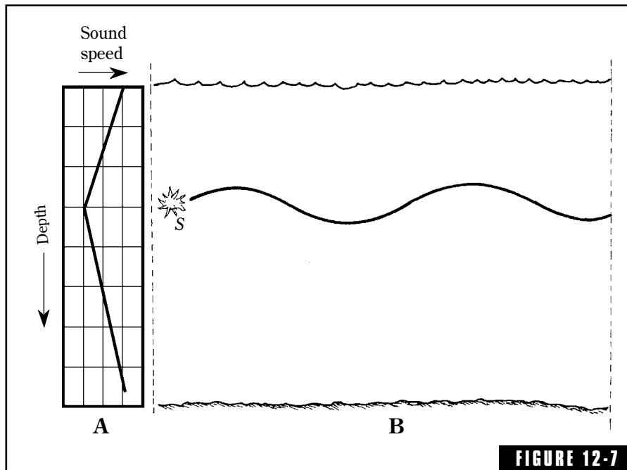
How the long range sound experiment of Fig. 12-6 was accomplished; (A) sound speed decreases with depth in the upper reaches of the ocean (temperature effect) and increases at greater depths (pressure effect) creating a sound channel at the inversion depth (about 700 fathoms). (B) A ray of sound is kept in this sound channel by refraction. Sound travels great distances in this channel because of the lower losses.
