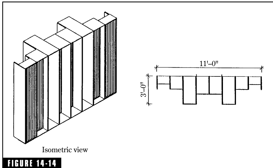
The large sized Model DFR-83LMH DiffRACTal™, a two-way system composed of a low-frequency unit (prime-7) with a mid-range DiffRACTal embedded at the bottom of each well. Peter D'Antonio, RPG Difusser Systems, Inc.
