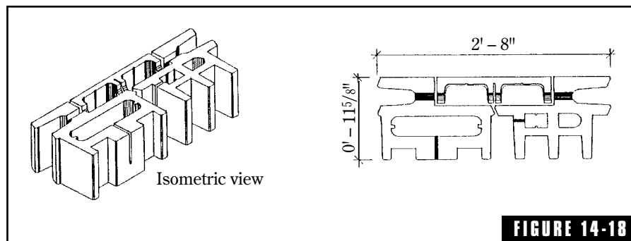
The DiffusorBlox™ concrete block, which offers the good transmission loss of a heavy wall, absorption via Helmholtz resonator action, and diffusion through quadratic residue action. The blocks are formed on standard block machines using licensed molds. Peter D'Antonio, RPG Diffusor Systems, Inc.
