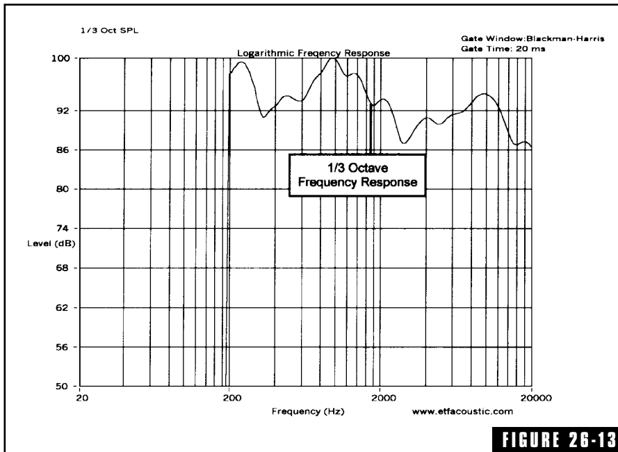
FIGURE 26-13 One-third octave frequency response measurement, with a 20-ms gate. (Courtesy of Doug Plumb, AcoustiSoft.)
