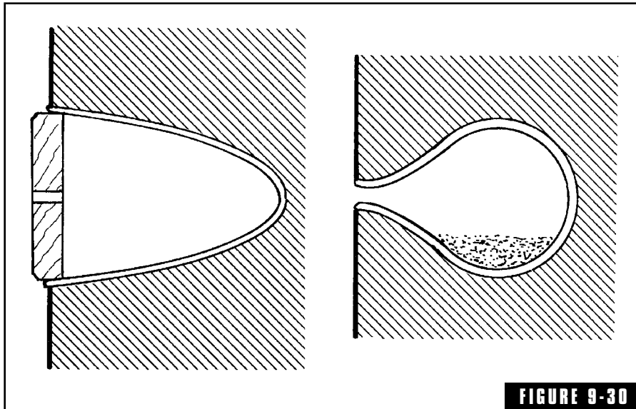
FIGURE 9-30 Pots embedded in the walls of medieval churches in Sweden and Denmark served as Helmholtz resonators, absorbing sound. Ashes, found in some of the pots, apparently served as a dissipative agent. (After Brüel. 11 )
