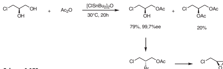
Scheme 1-175
