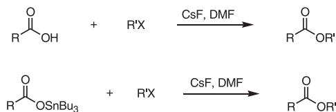
Scheme 3-15
