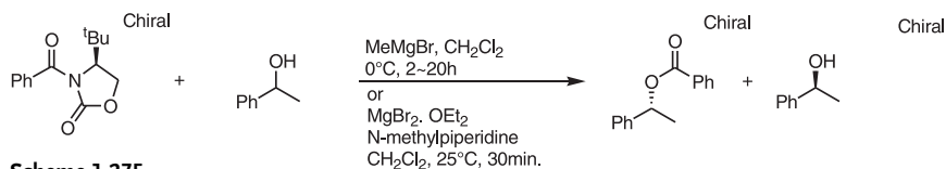
Scheme 1-275
