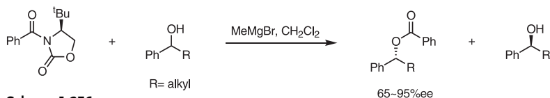
Scheme 1-276
