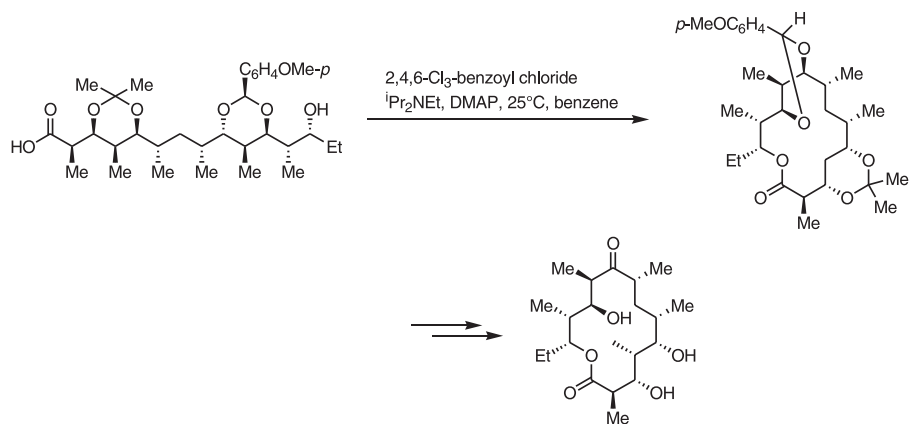
6-Deoxyerythronolide B
