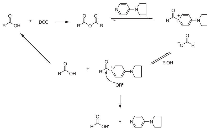
Scheme 1-25
