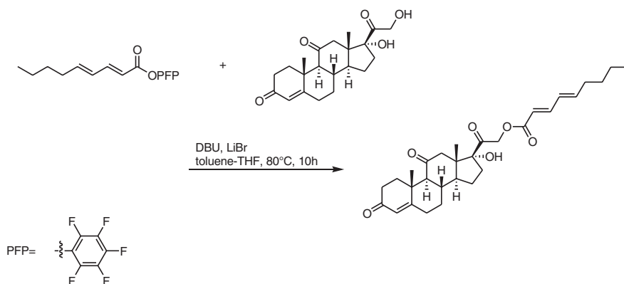
Scheme 1-133
