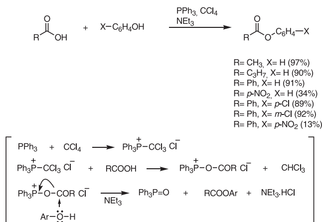
Scheme 1-45
