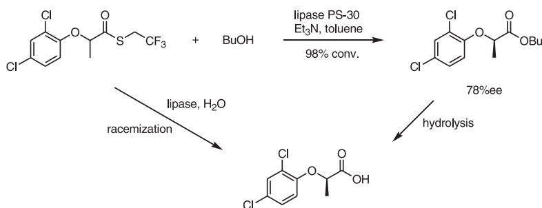
Scheme 5-4
