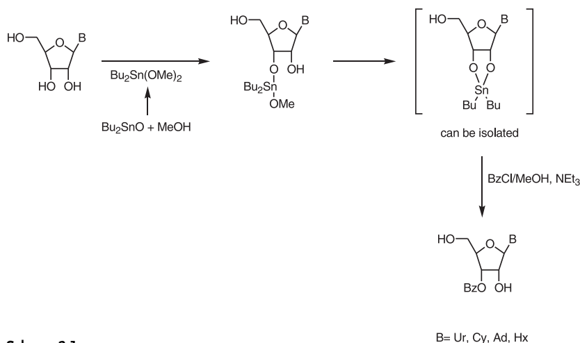
Scheme 2-1
