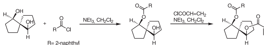
Scheme 1-259
