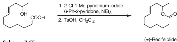
Scheme 7-65
