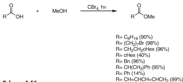
Scheme 1-56
