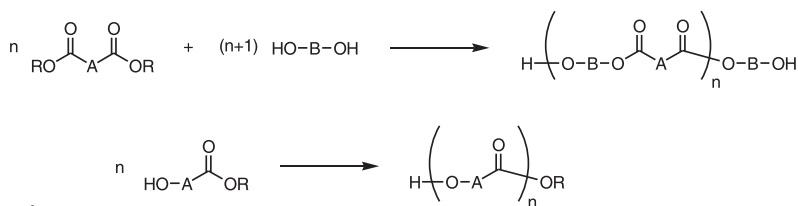
Scheme 8-1
