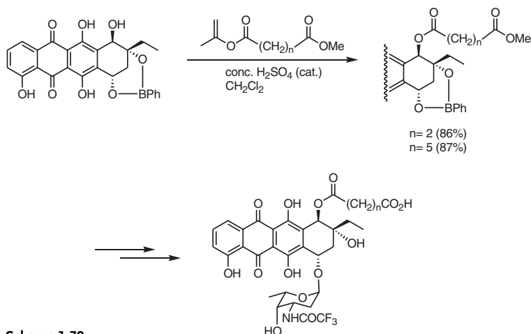
Scheme 1-79
