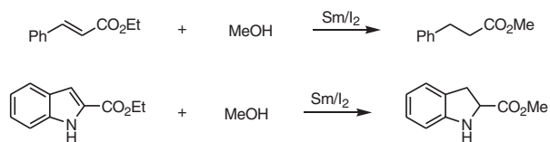
Scheme 1-143
