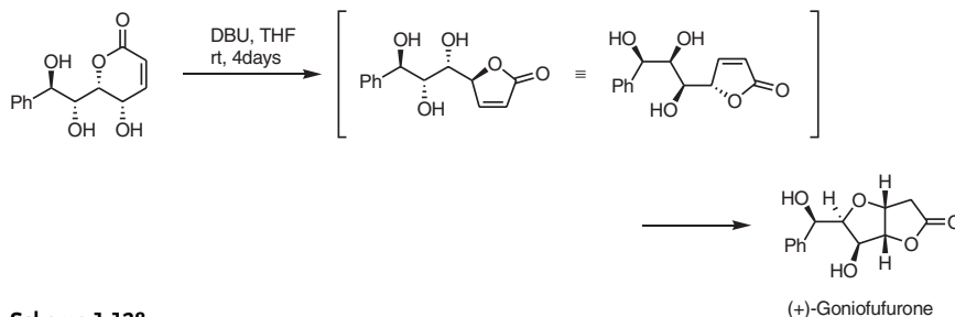
Scheme 1-128
