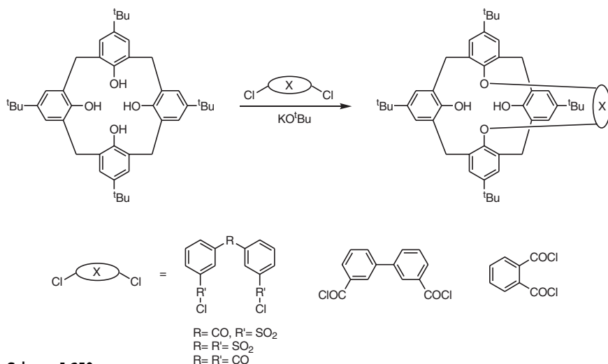
Scheme 1-250
