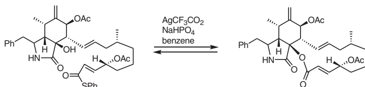
Scheme 1-243
