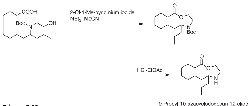
Scheme 7-66
