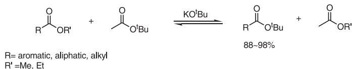
Scheme 4-2
