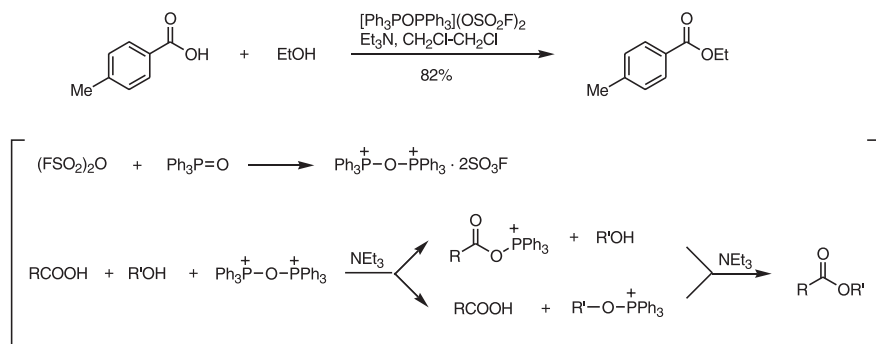
Scheme 1-48
