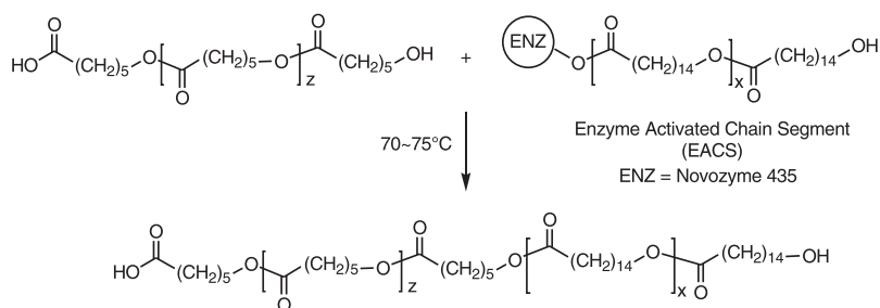
Scheme 1-153
