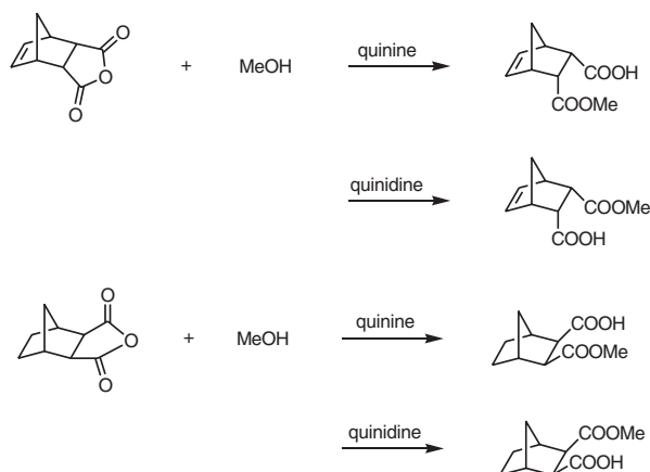
Scheme 1-207
