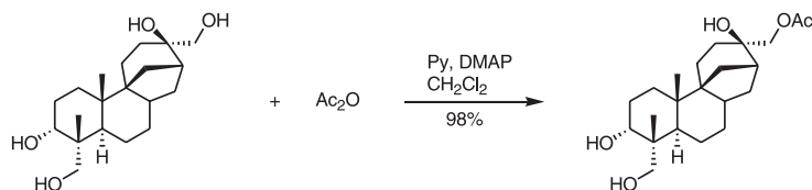
Scheme 7-17
