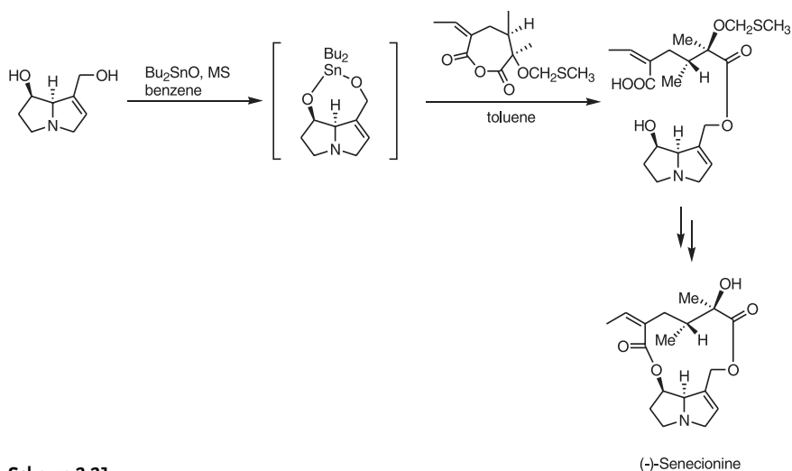
Scheme 2-21
