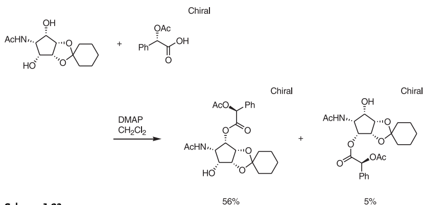
Scheme 1-23
