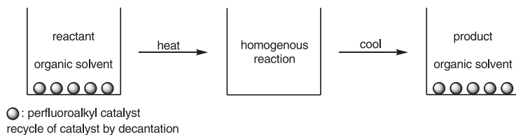
Scheme 7-49
