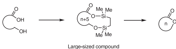
Scheme 1-51
