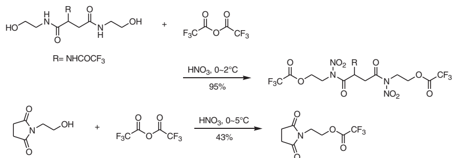
Scheme 1-163
