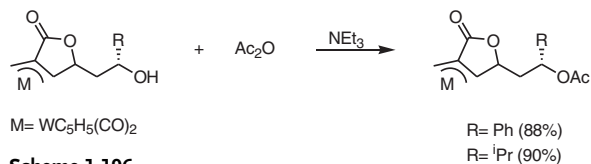
Scheme 1-196
