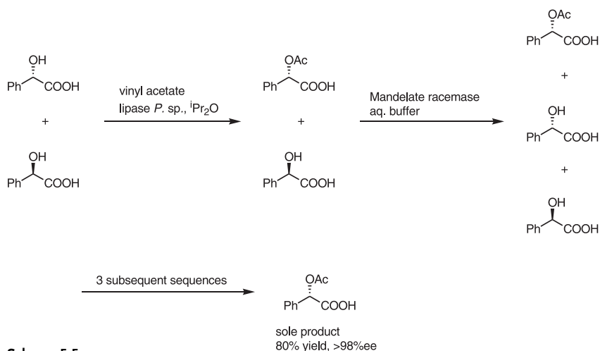
Scheme 5-5
