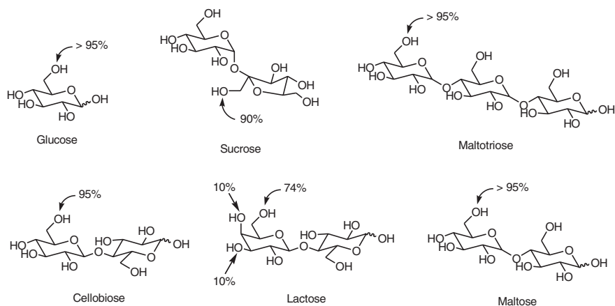
Scheme 1-157
