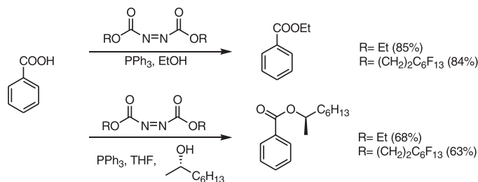
Scheme 7-50
