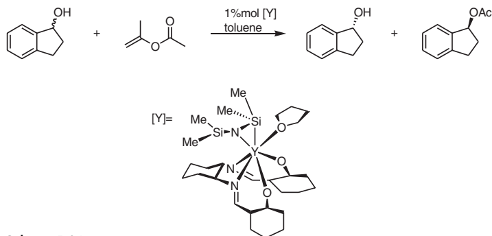
Scheme 1-94
