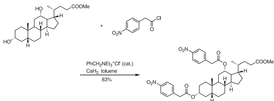
Scheme 7-39
