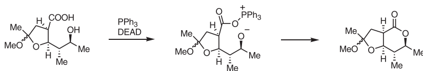
Scheme 1-30
