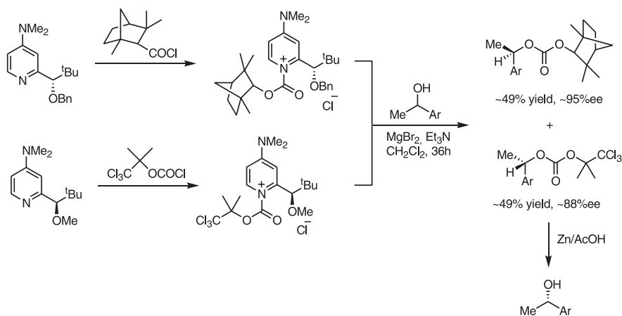
Scheme 5-12
