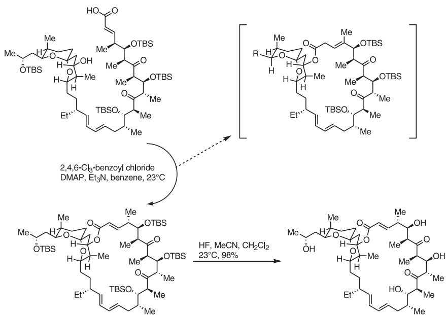
Scheme 7-58
