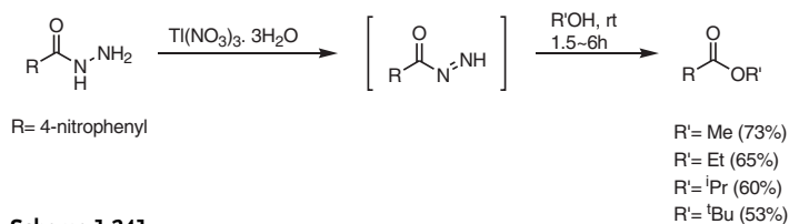
Scheme 1-241
