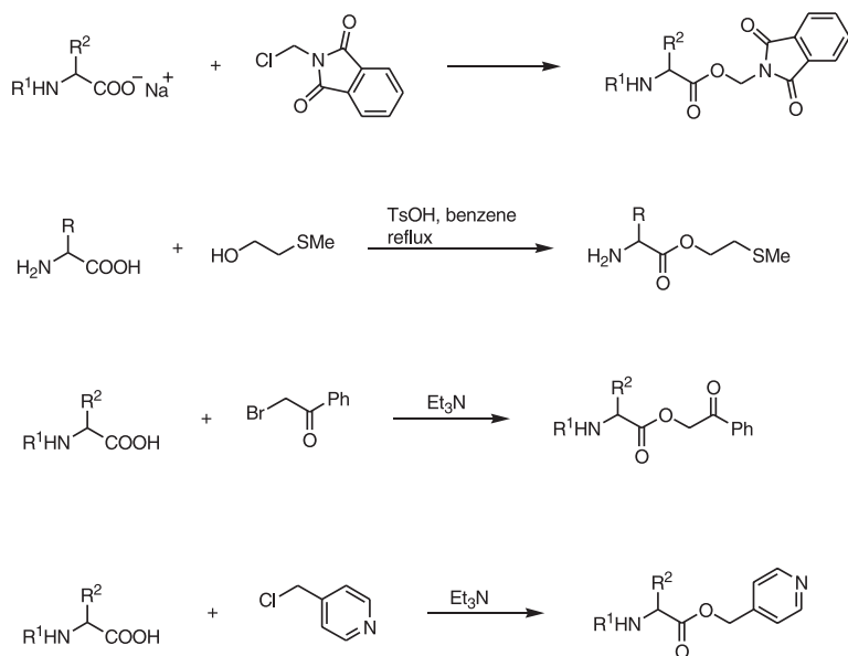
Scheme 8-12
