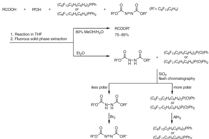
Scheme 7-51
