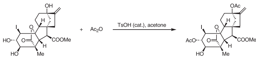
Scheme 7-35
