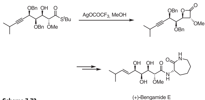
Scheme 7-72
