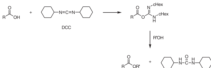
Scheme 1-24
