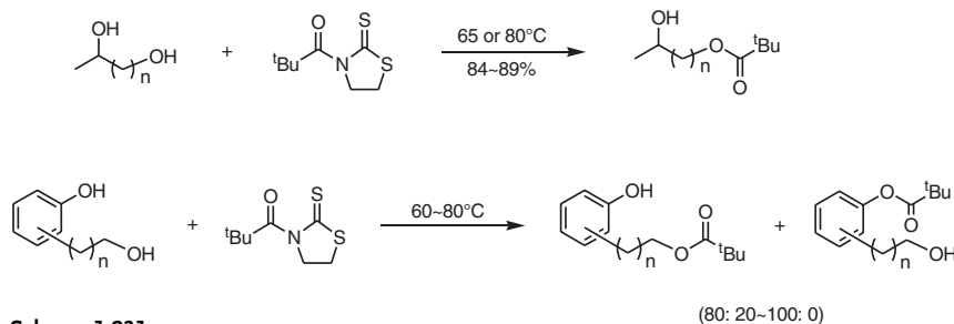
Scheme 1-231
