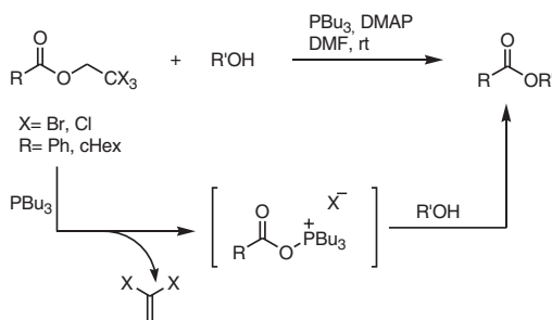
Scheme 1-140
