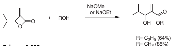
Scheme 1-113
