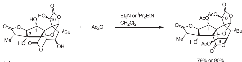
Scheme 7-37
