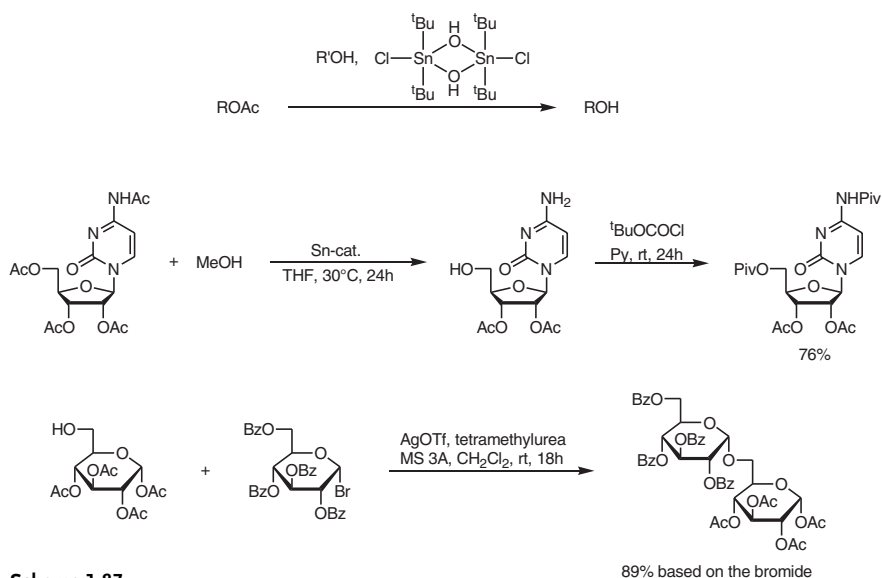
Scheme 1-87
