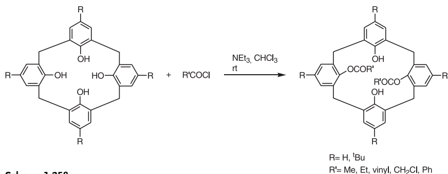
Scheme 1-258
