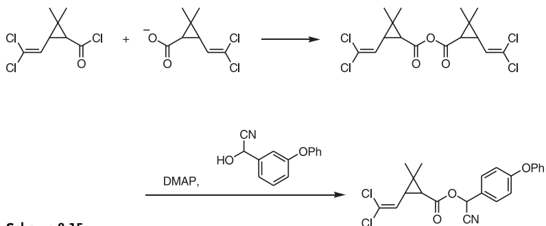
Scheme 8-15
