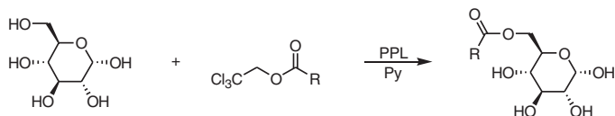
Scheme 1-144
