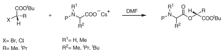
Scheme 3-11
