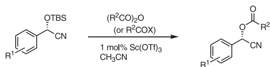
Scheme 1-167
