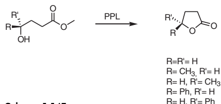
Scheme 1-147
