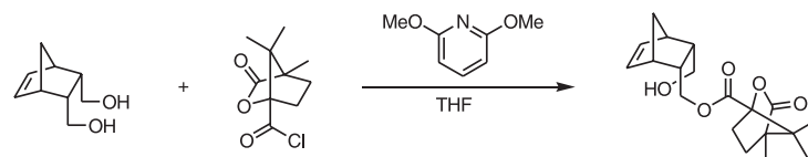
Scheme 6-5
