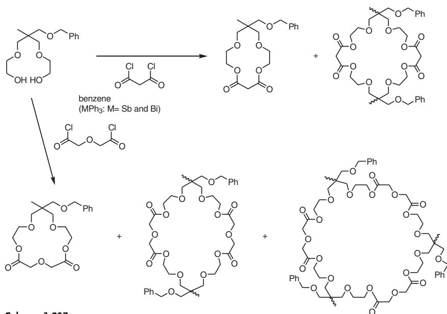
Scheme 1-237
