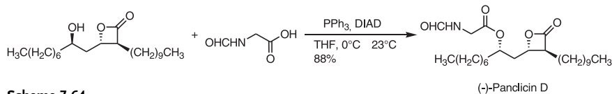
Scheme 7-64
