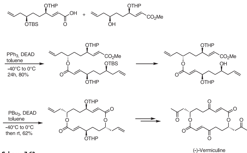
Scheme 7-63
