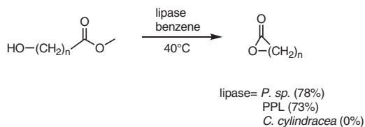
Scheme 1-146
