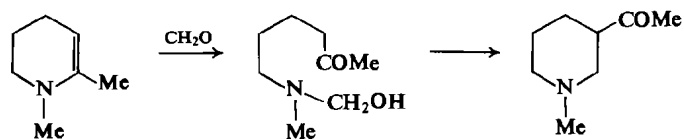
Scheme 18
