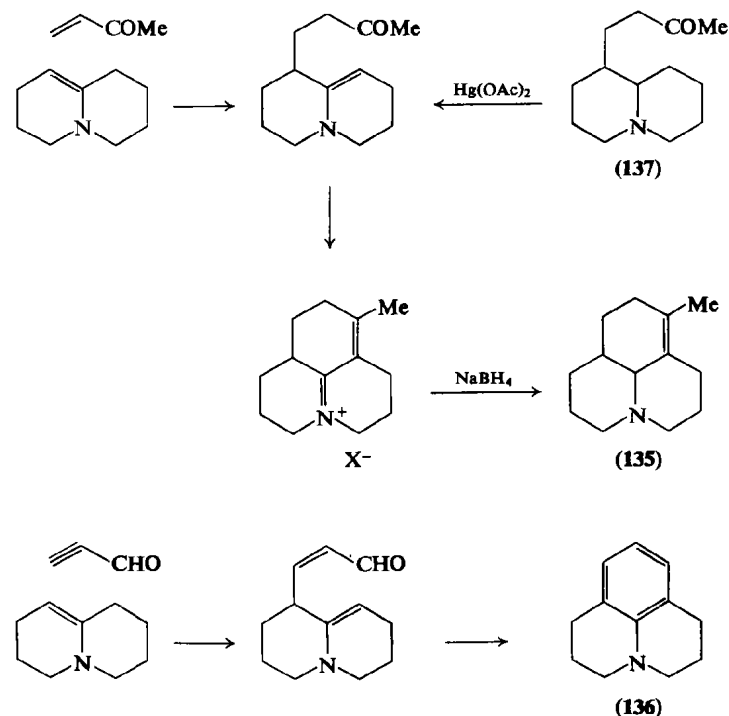
Scheme 11
