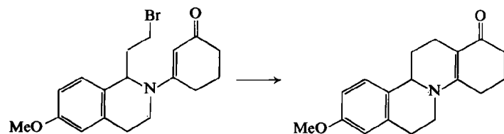
Scheme 6
