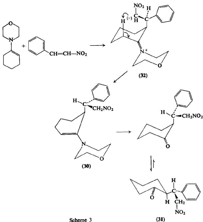
Scheme 3
