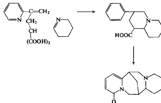
Scheme 20
