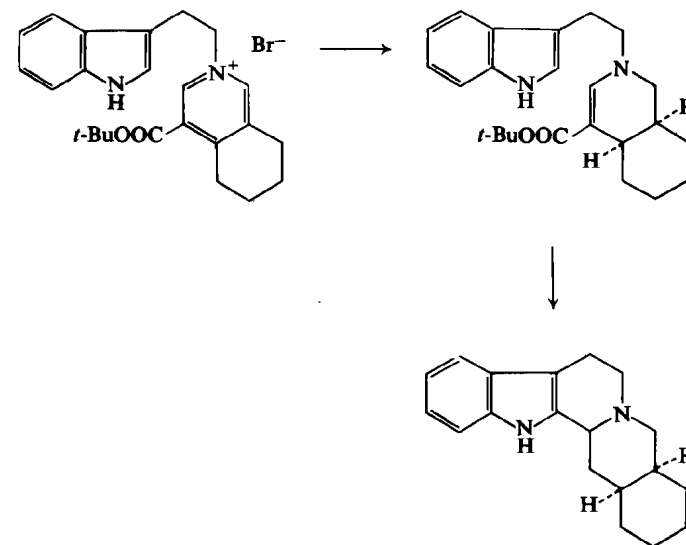
Scheme 21
