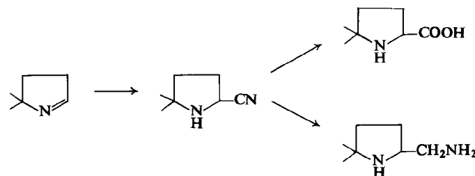
Scheme 15
