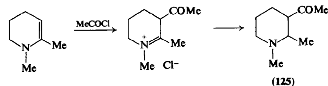
Scheme 8
