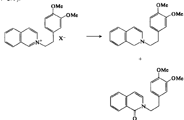
Scheme 16
