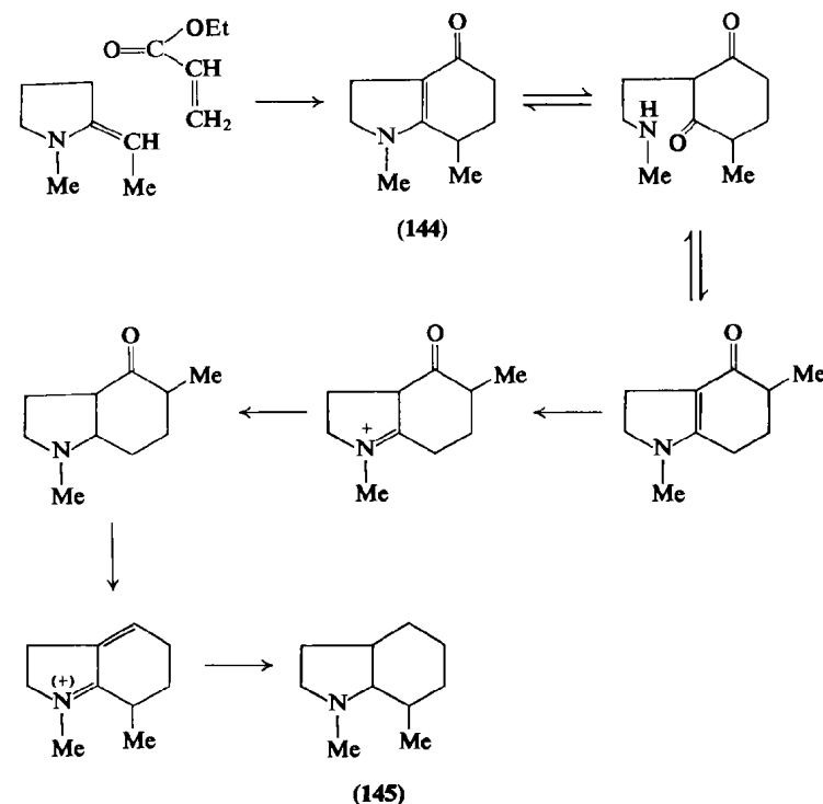
Scheme 12
