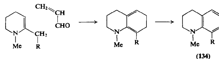
Scheme 10
