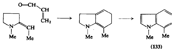
Scheme 9
