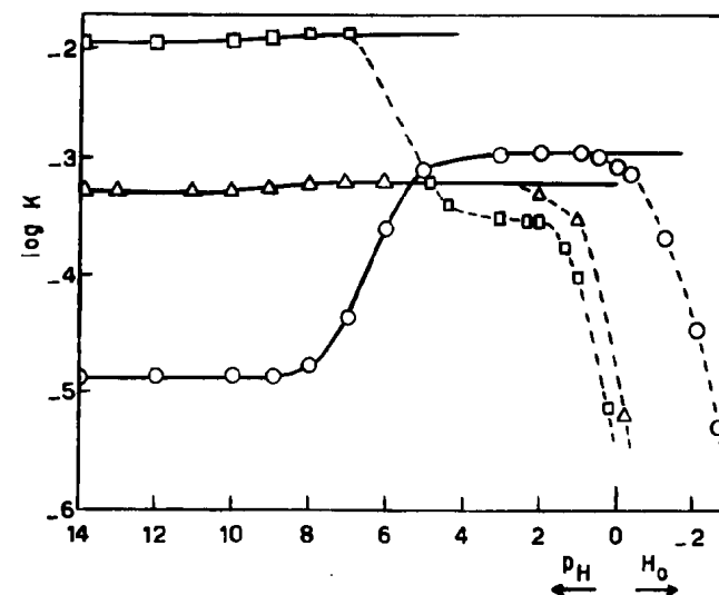
Fig. 2. Observed vs. calculated rates of hydrolysis of enamines at 24.8°. Drawn lines: calculated \log k values. Observed values: \circ for 4-(2-methylpropenyl)morpholine; \triangle for 1-(2-methylpropenyl)piperidine; \square for 1-(2-methylpropenyl)pyrrolidine. Values are corrected for buffer contributions (23).
