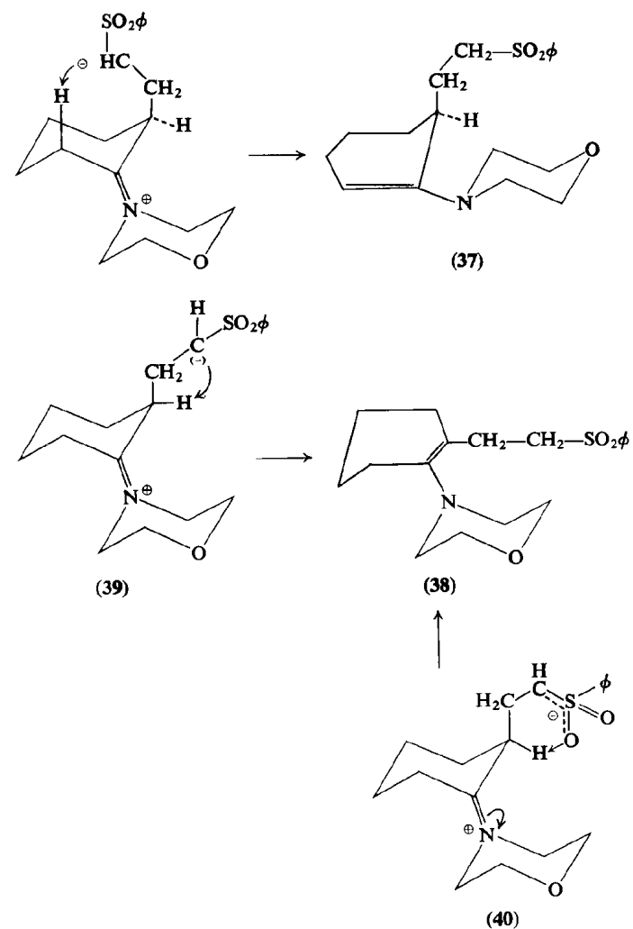
Scheme 4
