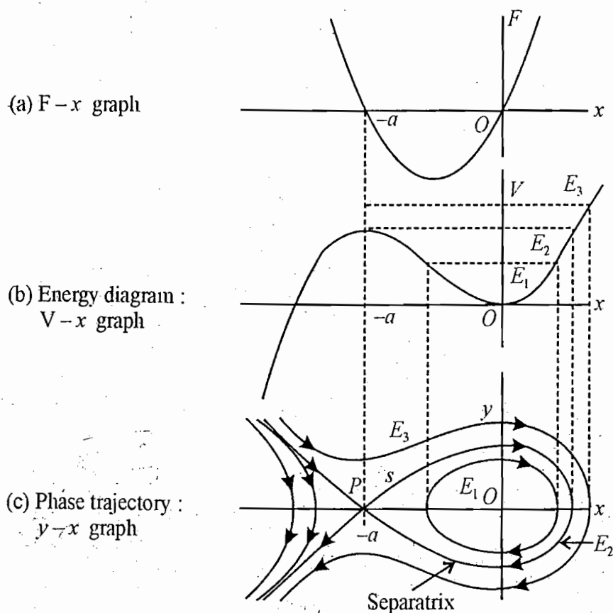
Fig. 16.7. Phase trajectory corresponding to equation F(x) = x(x+a)
