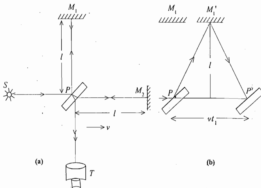
Fig. 12.3 : Michelson-Morley Experiment
