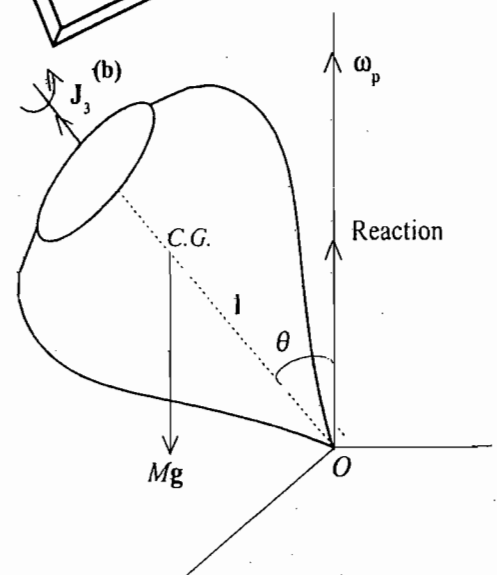
Fig. 10.22 : Precession under gravitational torque.
