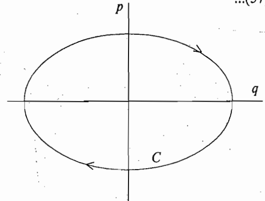
Fig. 8.1 : Phase path for one-dimensional harmonic oscillator ... (58a)
