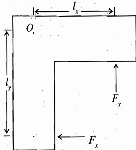
Fig. 13.4 : Equilibrium of a right-angled lever
