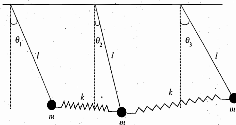
Fig. 9.21. Triple pendulum
