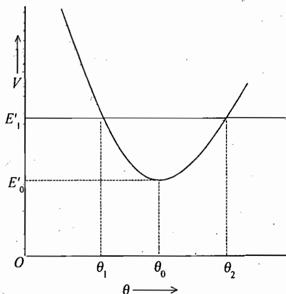
Fig. 10.19 : Plot of effective potential V(\theta) versus \theta ( 0 \leq \theta \leq \pi ) for a heavy symmetrical top
