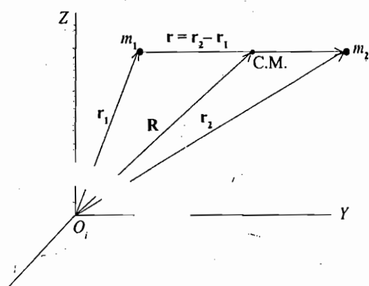
Fig. 4.1. Two-body problem : relative and centre of mass coordinates
