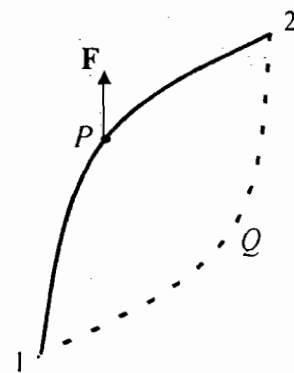
Fig.1.4 : Work done by a force on a particle
