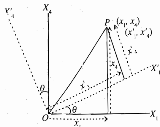
Fig. 14.1 : Rotation of orthogonal coordinates axes and invariance of OP^2 = x_1^2 + x_4^2 = x_1'^2 + x_4'^2
