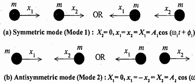
Fig. 9.3 : Normal modes of two coupled masses
