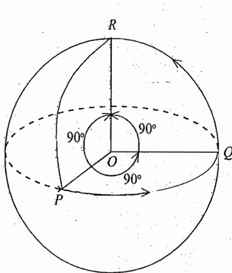
Fig. 10.7. Finite rotation cannot be represented as vector
