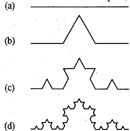
Fig. 16.30. Koch curve
