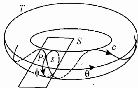
Fig. 16.33. Invariant 2-torus, showing surface of section S : the trajectory e generates poincare section s .
