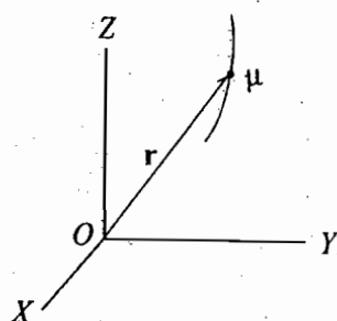
Fig. 4.2 : Reduction of two-body problem to one-body problem
