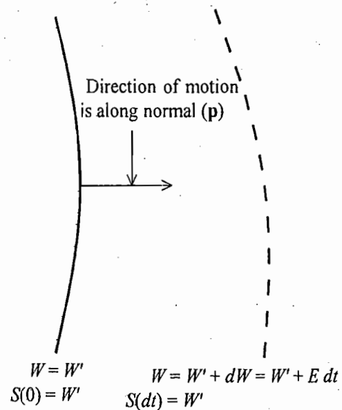
Fig. 8.2 : The Motion of the Surfaces of constant S in Configuration space
