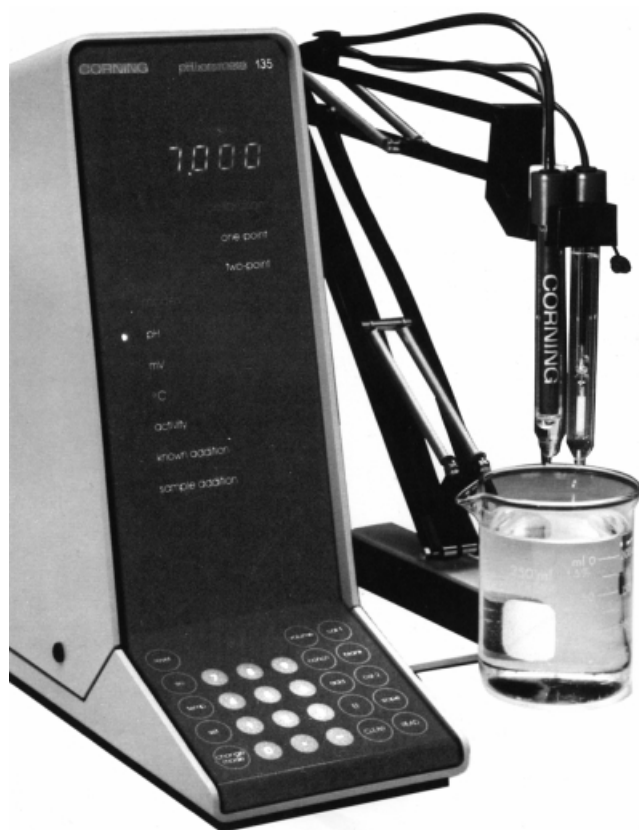
FIGURE 5-8 A modern microprocessor-controlled pH meter.
